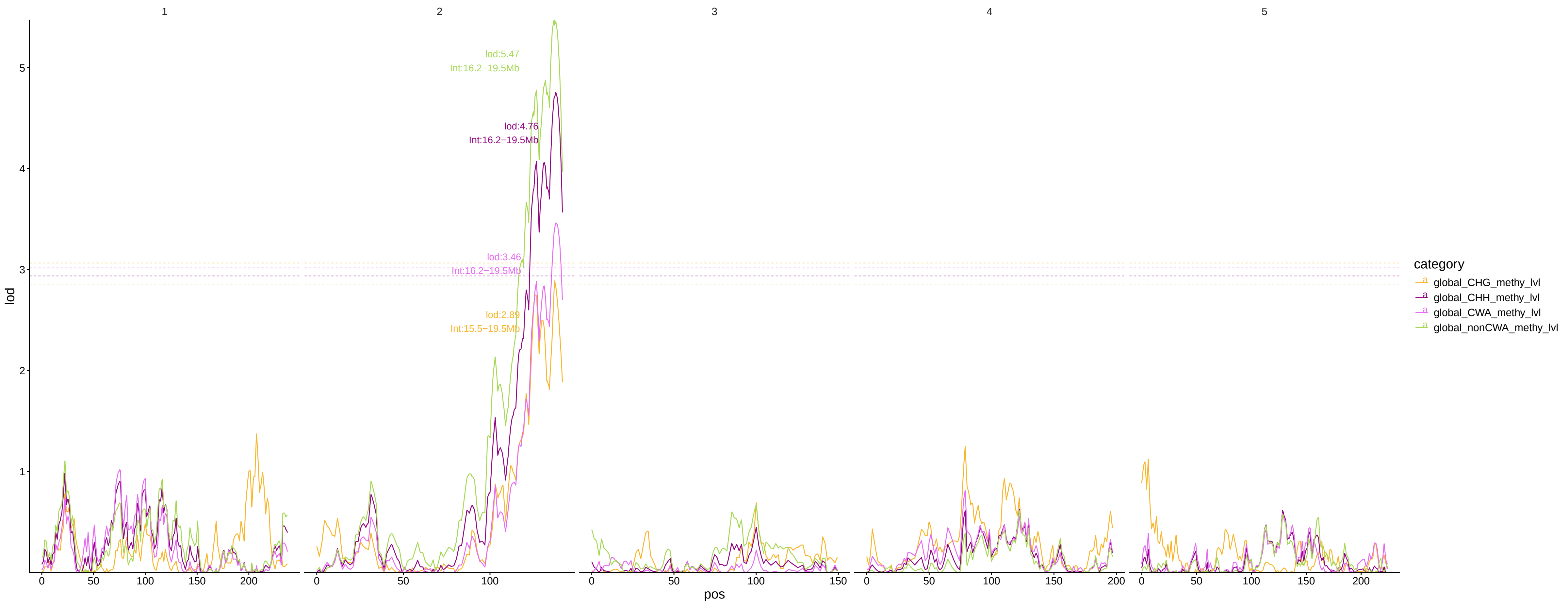
global CHG & CHH & CWA & nonCWA new methy level
